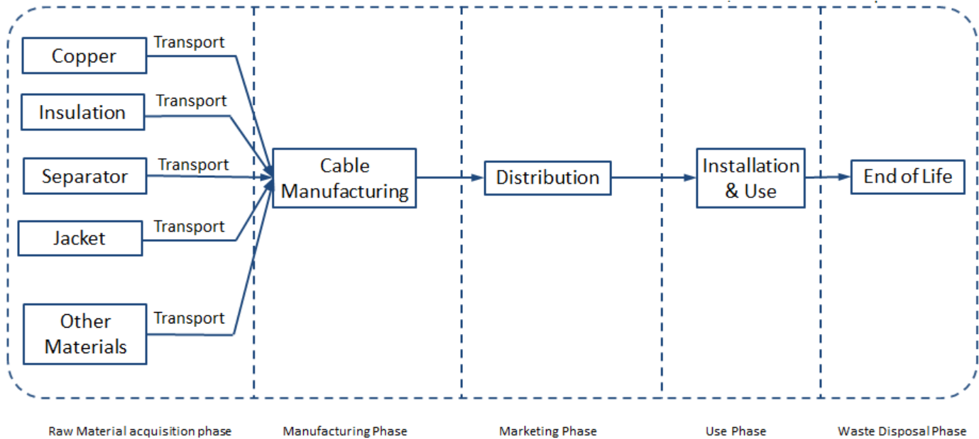
Figure 3: System Boundary
